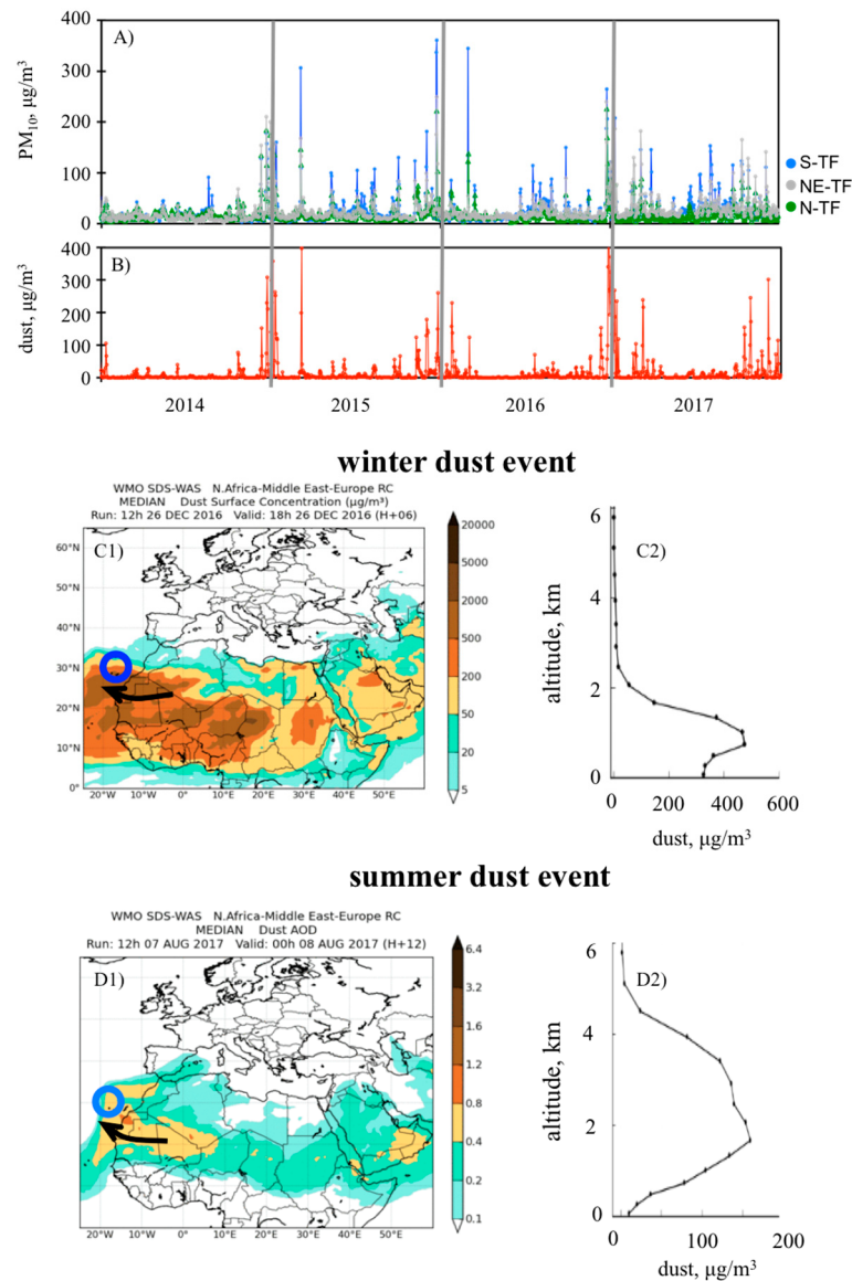
Figure 2. Time series of daily mean values of (A) PM_{10} measured at three sites of Tenerife (South, S-TF; Northeast, NE-TF; and North, N-TF) and of (B) surface dust concentrations provided by the World Meteorological Organization's Sand and Dust Storm Warning Advisory and Assessment System (WMO SDSWAS). Example of a typical dust event of winter (26-Dec-2016): surface dust concentrations (C1) and vertical dust profile in Tenerife (C2). Example of a typical dust event of summer (08-Aug-2017): dust optical depth (D1) and vertical dust profile in Tenerife (D2). Blue circle highlights the location of Tenerife.
